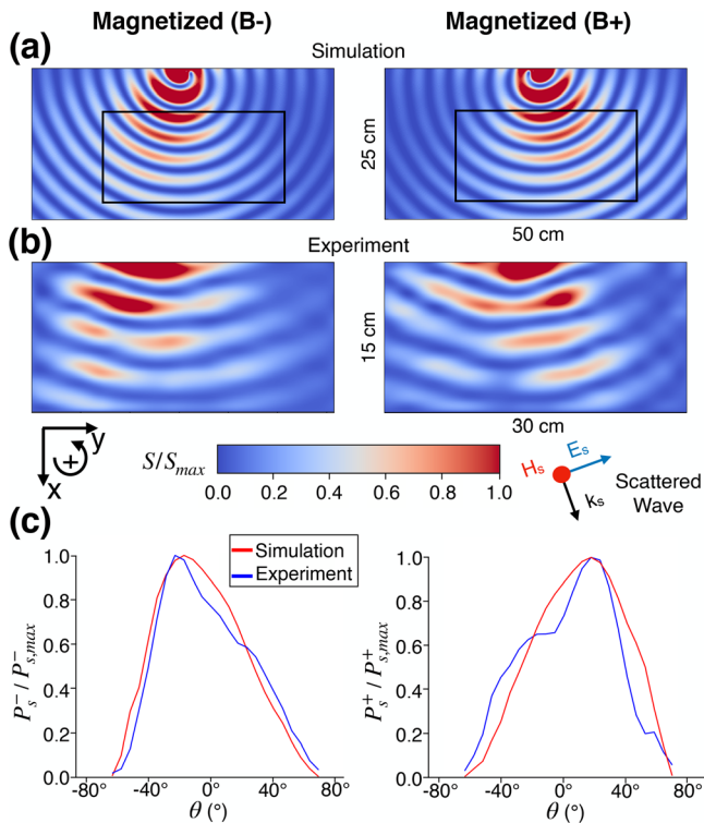
FIG. 3. Normalized Poynting vector of a 4.42 GHz scattered wave from a magnetized plasma rod: (a) simulated using CST and (b) experimentally measured in the 15 \times 30 cm 2 region represented by the black rectangle. (c) Normalized scattered power derived from experiments and simulations in the black rectangle region at 4.42 GHz.
